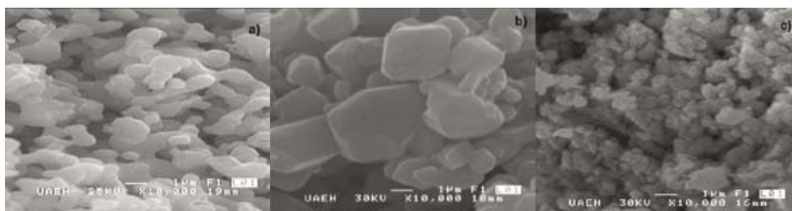
Figure 2. Scanning electron micrographs of \text{Eu}_x\text{Ca}_{1-x}\text{MnO}_3 manganite: a) x = 0 , b) x = 0.05 , c) x = 0.30 .
