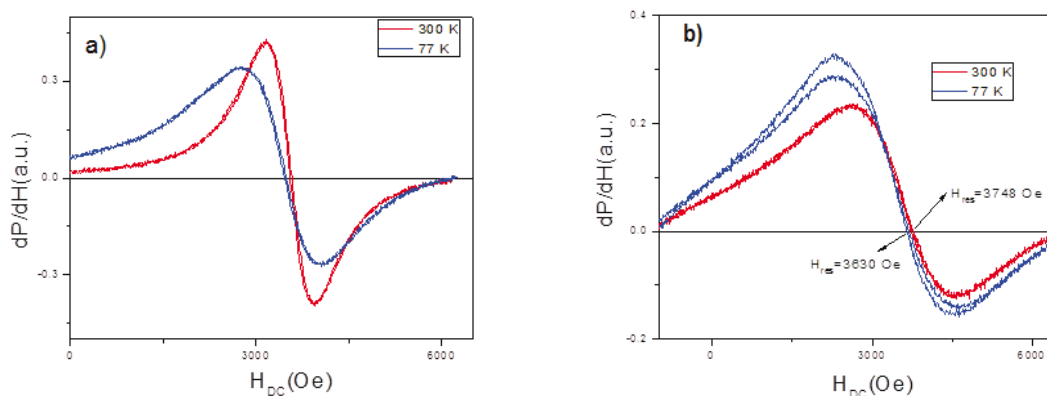
Figure 4. EPR spectra of a) \text{CaMnO}_3 and b) \text{Eu}_{0.30}\text{Ca}_{0.70}\text{MnO}_3 manganite at 300 and 77 K.
