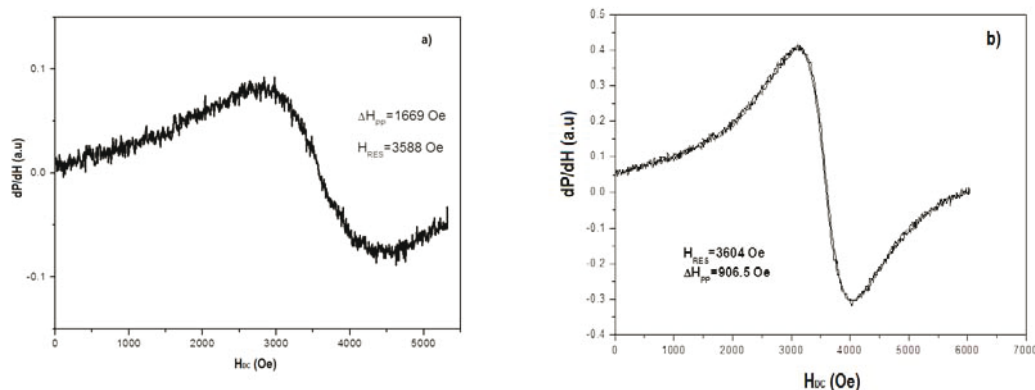
Figure 3. EPR signals at 300 K, a) \text{CaMnO}_3 , b) \text{Eu}_{0.05}\text{Ca}_{0.95}\text{MnO}_3 manganite.
