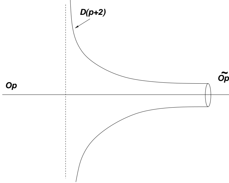
Figure 4: Brane realization of \widetilde{O}p -planes.
