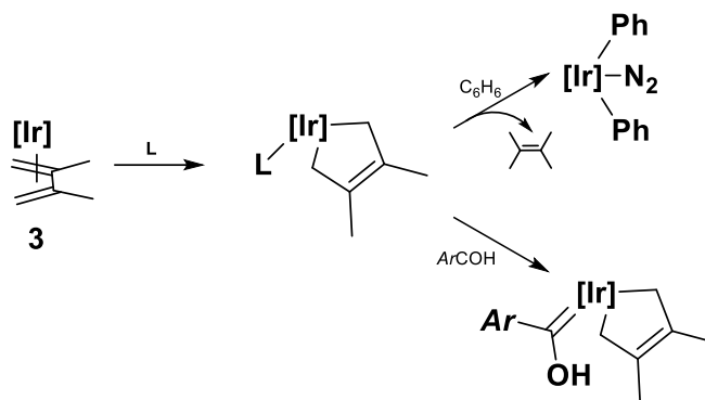
Esquema 5. Reactividad del complejo [\text{Tp}^{\text{Me}_2}\text{Ir}(\eta^4\text{-CH}_2=\text{C}(\text{Me})\text{C}(\text{Me})=\text{CH}_2)] .
