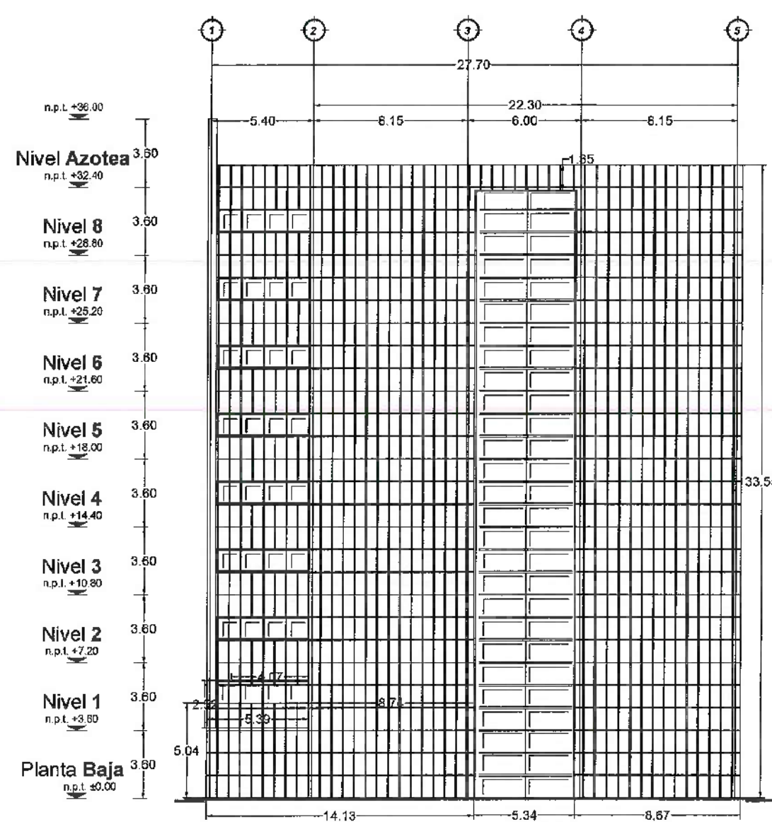
FACHADA PRINCIPAL NORTE
